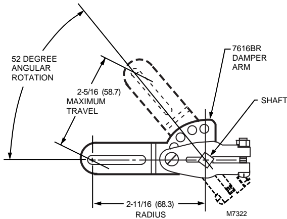
Fig. 3. 7616BR Damper Crank Arm can be attached to actuator shaft to drive a damper at same time valve is opened.
