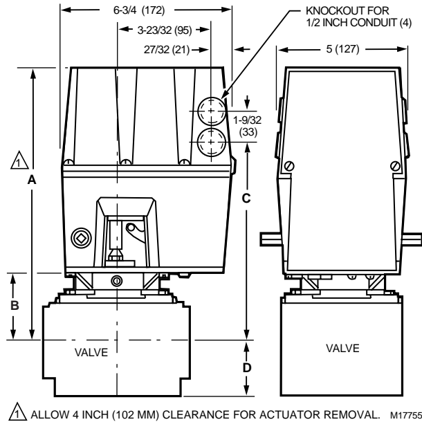
Fig. 1. Approximate mounting dimensions of V4062 Actuators in in. (mm).
